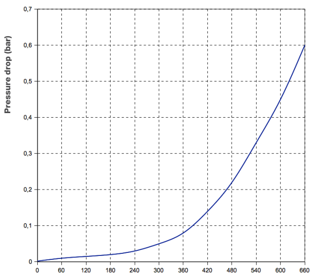
Pressure drop at type AB-F50
